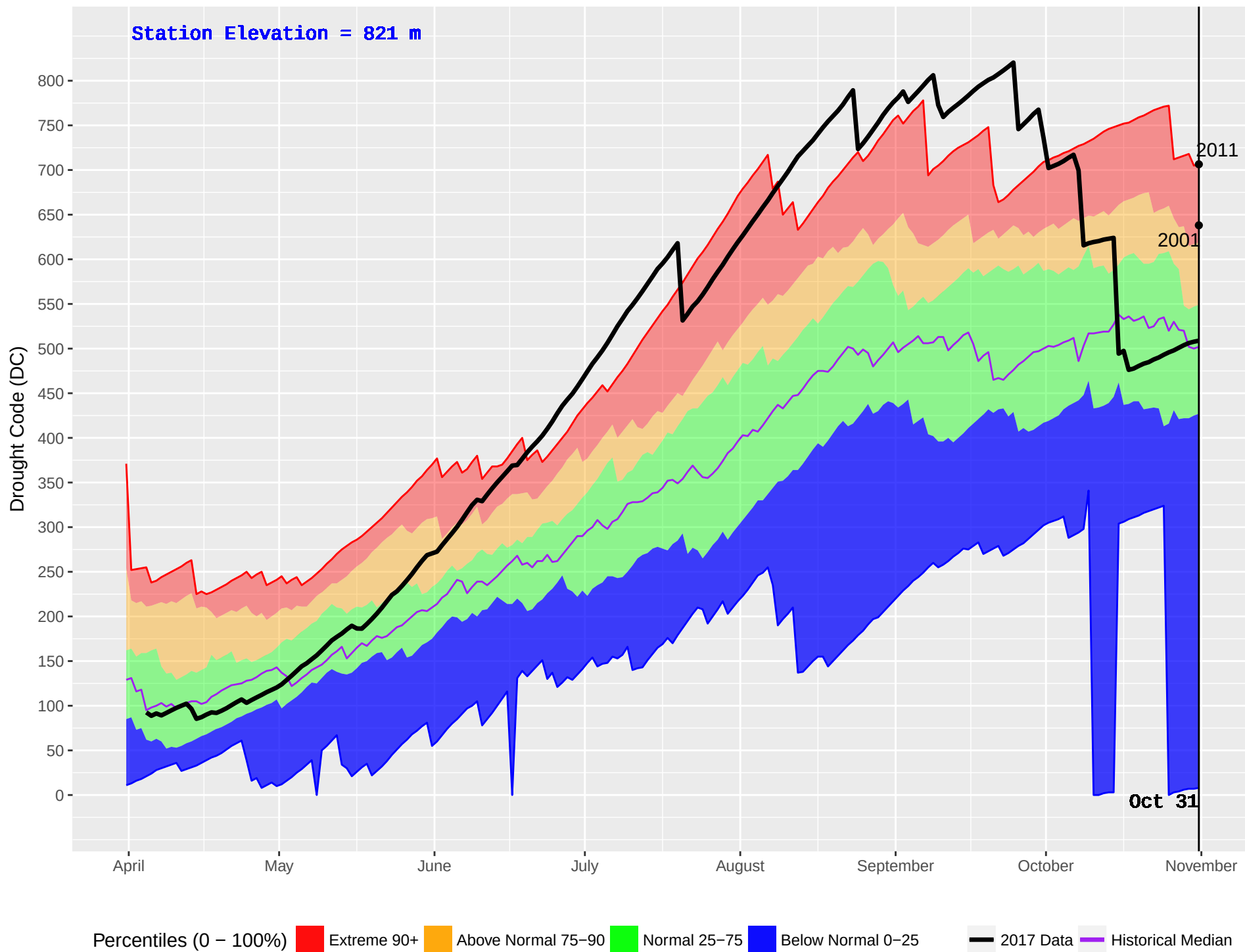
KNIFE (225) : Historical (1991–2016) and Current (2017) Noon Drought Code (DC)
