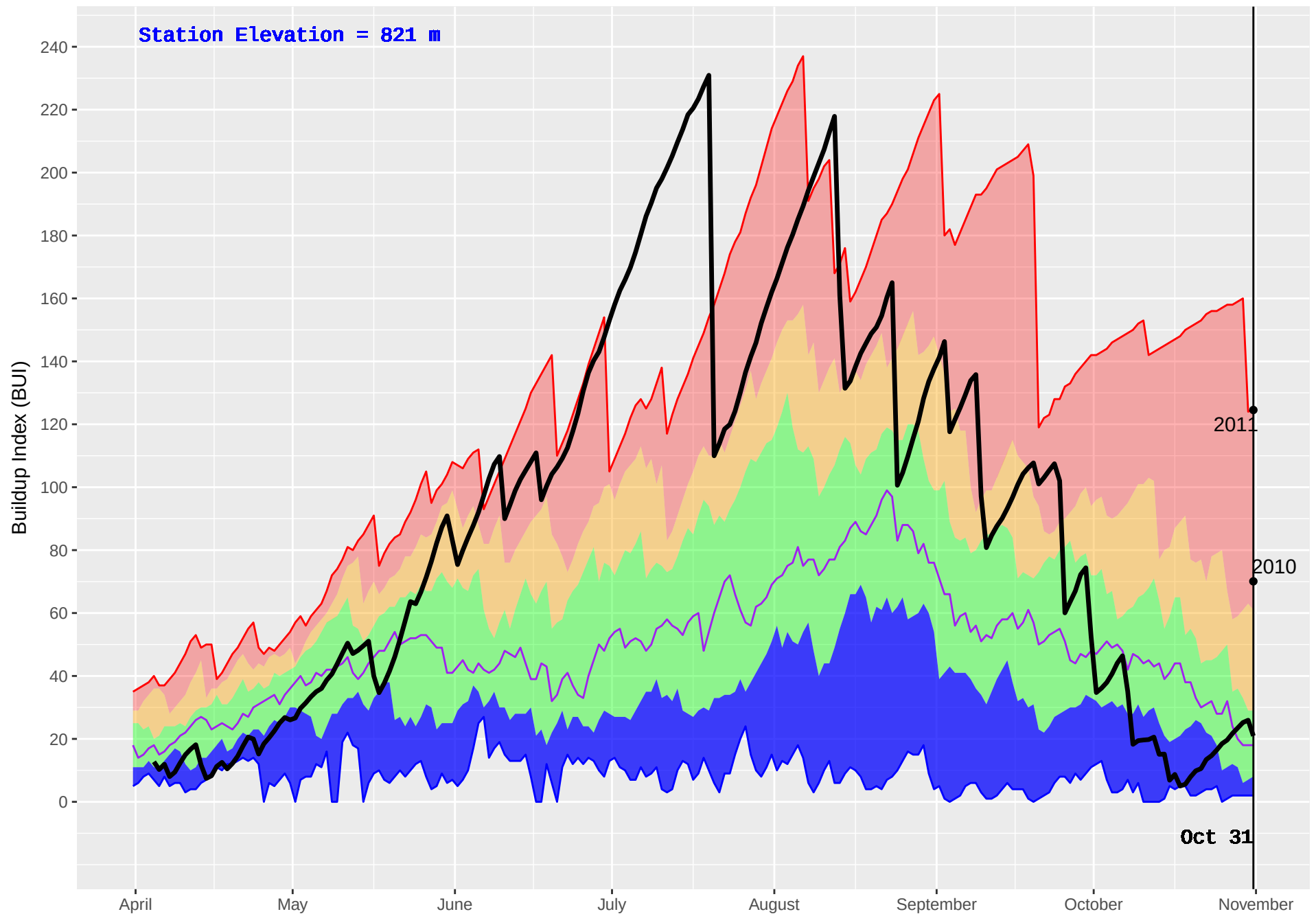
KNIFE (225) : Historical (1991–2016) and Current (2017) Noon Buildup Index (BUI)
